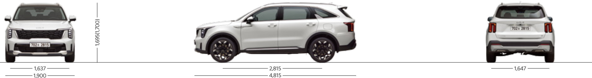
※ Wheel tread: Corresponds to 20" tires / ※ Overall height: "( )" includes the roof rack Units: mm
